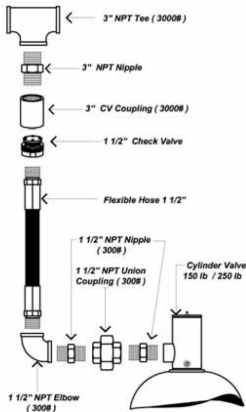
1 1/2" Check Valve Installation (Screwed Type CV Coupling)
