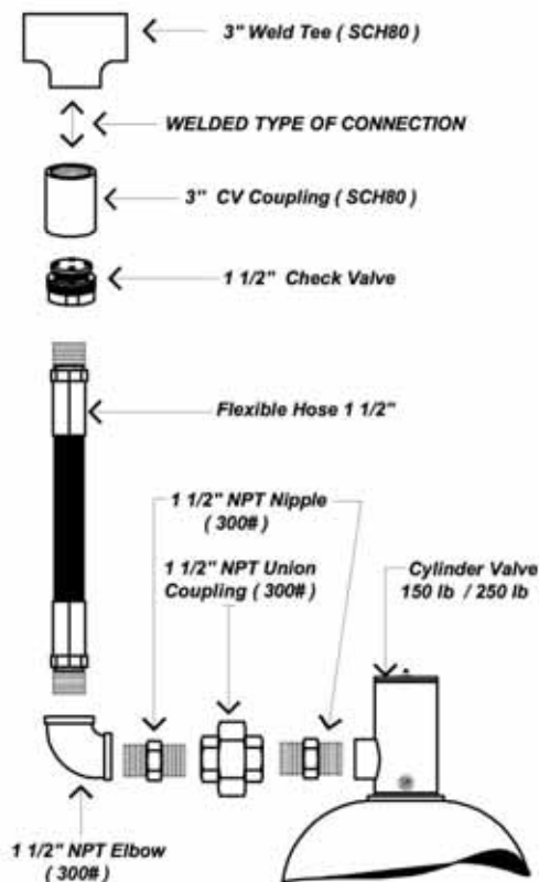
1 1/2" Check Valve Installation (Welded Type CV Coupling)
